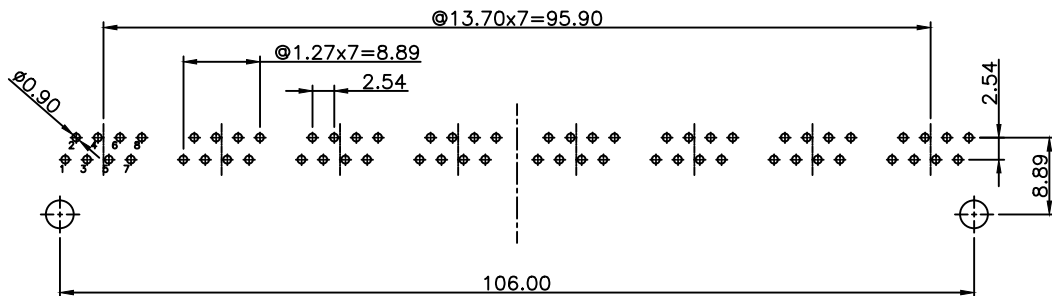
PC Board Layout Component Side Shown PC Board Thickness=1.6mm Tolerance±0.05
